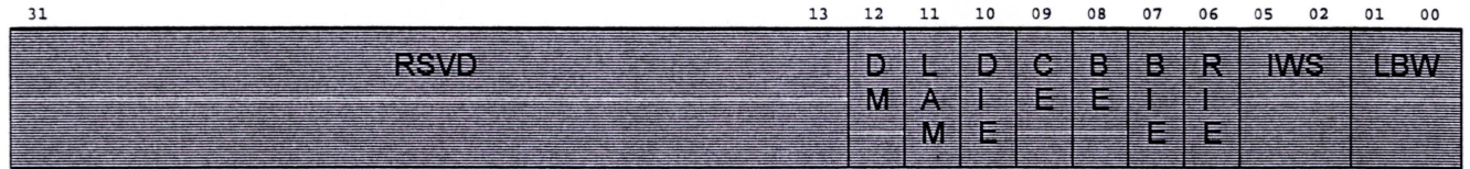
Figure D-7: DMA Channel 1 Mode Register
