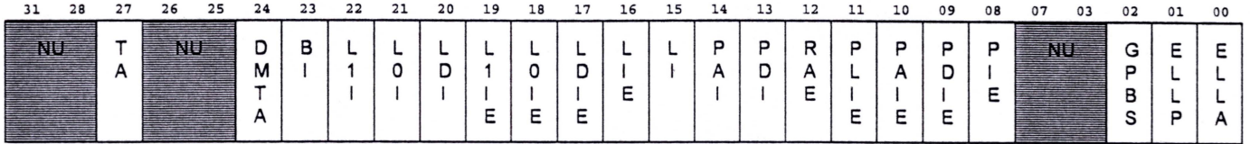
Figure 4-36: Interrupt Control/Status Register
