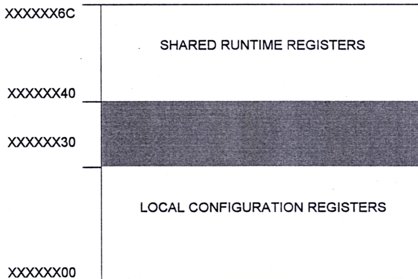
Figure 3-1: PCI Control Address Space
