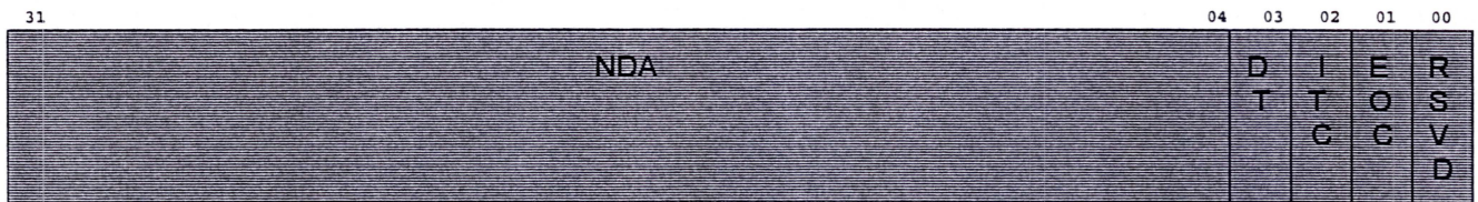
Figure D-6: DMA Channel 0 Descriptor Pointer Register
