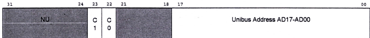
Figure 4-48: Unibus Address Register
