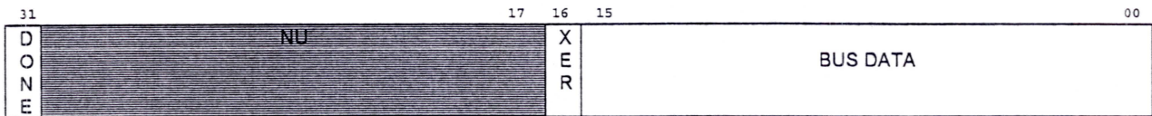
Figure 4-44: Bus Data Register
