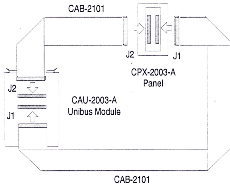
Figure 1-4: Installing Ribbon Cables
