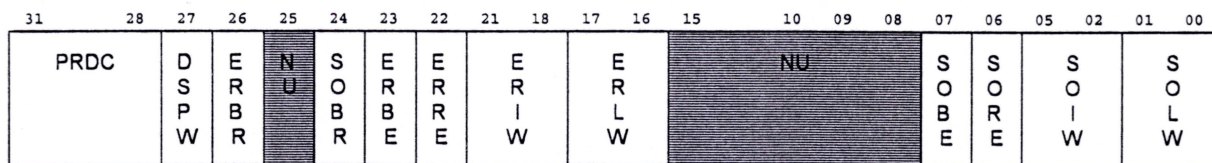
Figure 4-26: Local Region Descriptor Register
