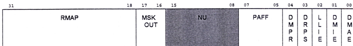
Figure 4-30: Direct Master Control Register
