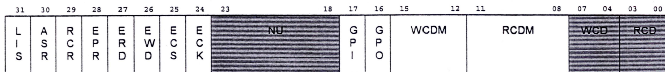
Figure 4-37: EEPROM PCI I/O Control Register
