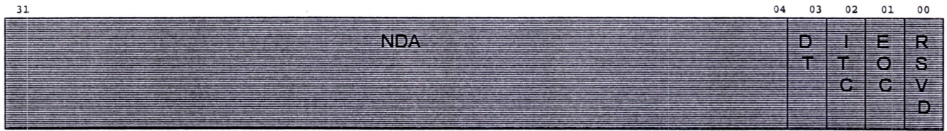
Figure D-11: DMA Channel 1 Descriptor Pointer Register
